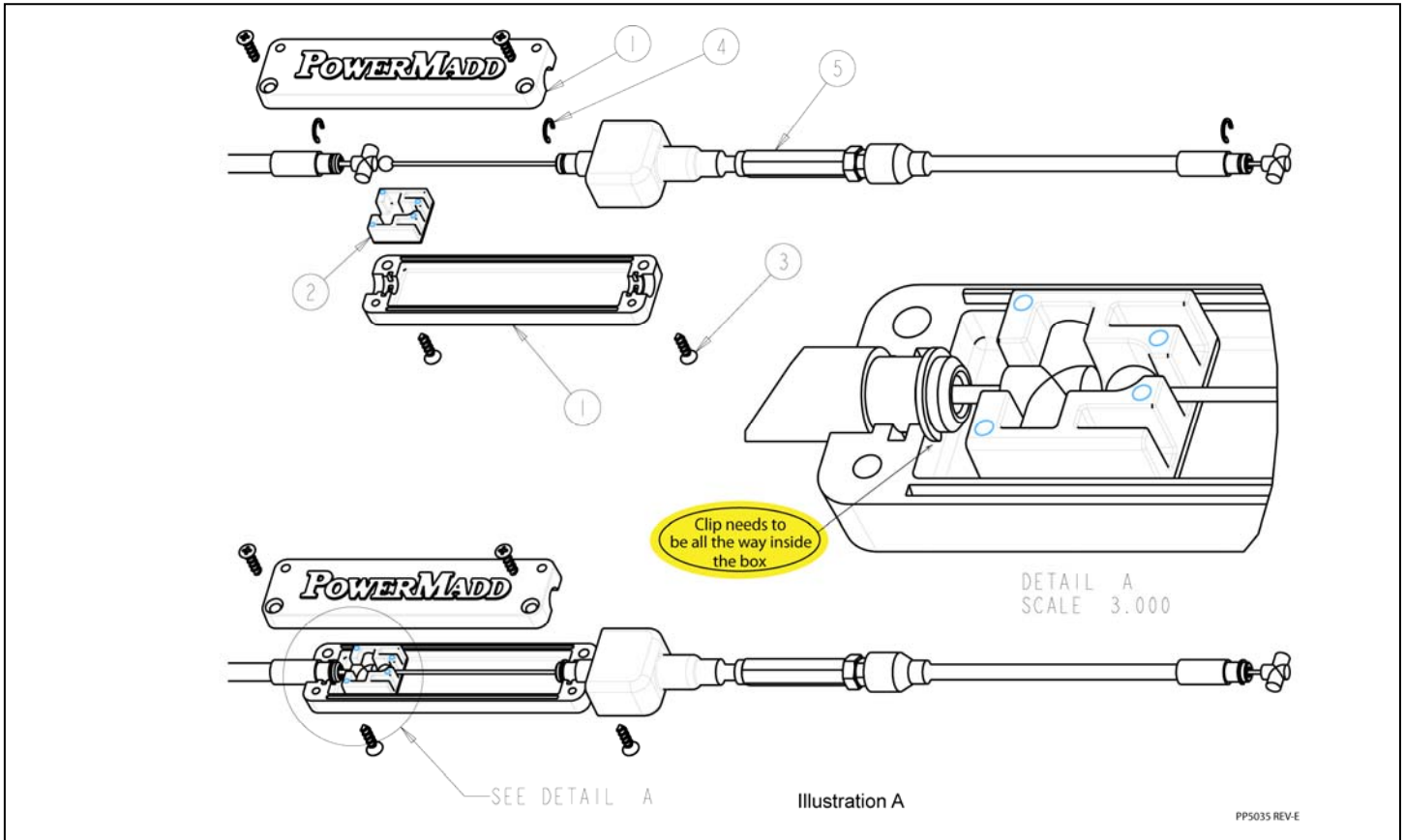
PM13592 - PowerMadd Throttle Cable Extension Junction Box Detail
